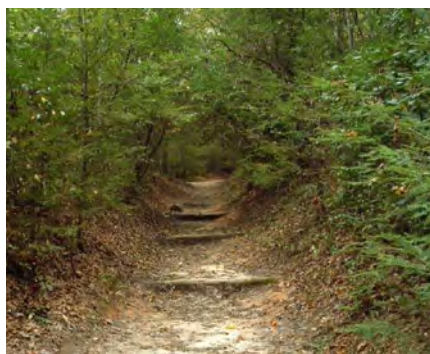
Figure 5-32. Water bars installed on bare earth trail (Northeast Avalon Atlantic Coastal Action Program).
