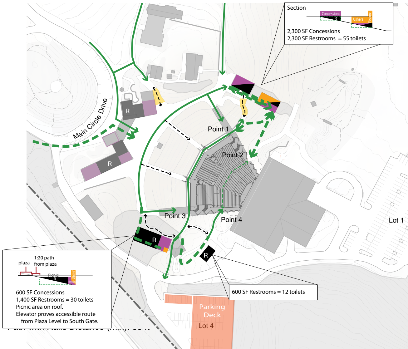
Figure 6-13. Filene Center Detail Area Option 1 Proposed access and program
