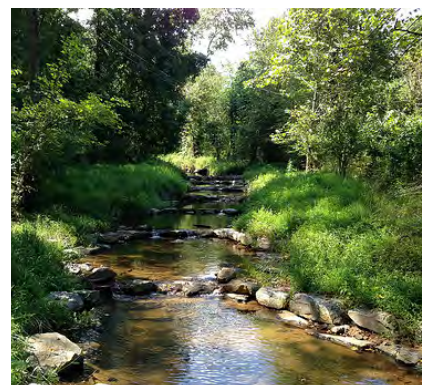
Figure 5-6. Step pools are constructed in the stream channel to recreate natural channel morphology. As flow moves over the step, energy is dissipated into the pool (source: Montgomery County, MD "Stream Restoration Techniques").
