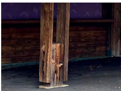
Figure 5-46. Timber structure, Stand A. (QE, 2020).
