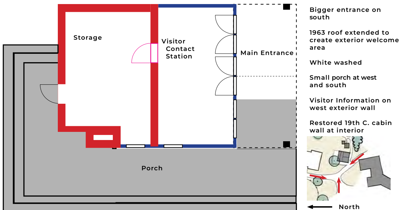
Figure 6-35. Proposed Cabin floor plan to transform it into a Visitor Contact Station.
