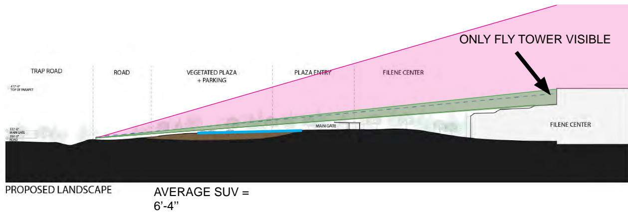
Figure A-3. Grading for parking within the dimple and the height of cars within this space would block views of all but the Filene Center fly tower from the Main Circle Drive (QE and Gensler).
