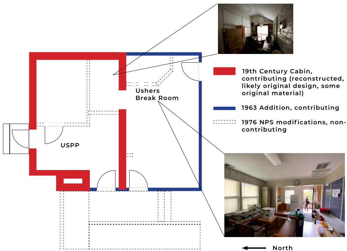
Figure 6-34. Existing Cabin floor plan diagram showing era of construction.
